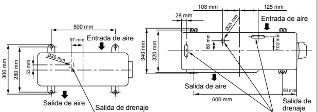
RAS-05, 07, 10, 13J2AVG-E
