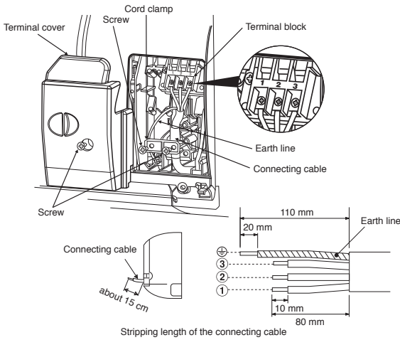
Stripping length of the connecting cable
