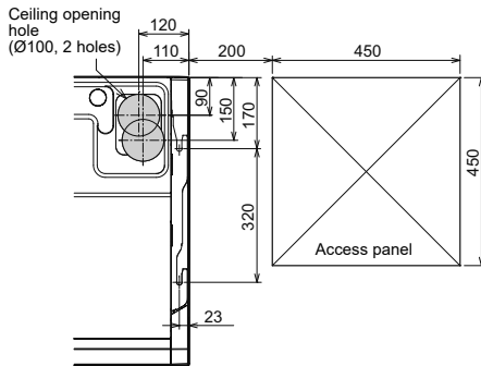
Position of ceiling opening hole
