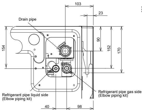
Position of refrigerant pipes and drain pipe
