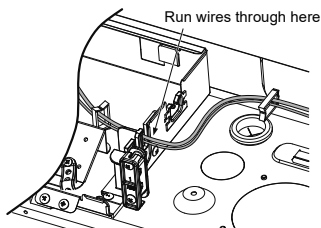
Position of connectors on indoor unit P.C. board
